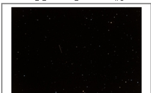
asteroid_2004_b186_20150127_1401288715.jpg
