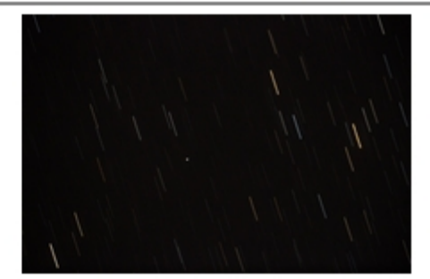
asteroid_2004_b186_20150127_1363626400.jpg
